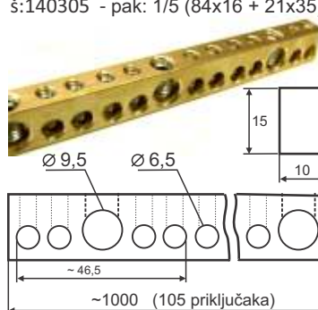
Stezaljka 105 x 16-35mm 2 200A š:140305 - pak: 1/5 (84x16 + 21x35)
